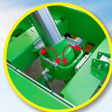
Telescopic tipping cylinder on a double oscillating frame placed in a forward position in the chassis
