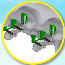
Bolted and movable Hydro-Tandem running gear
