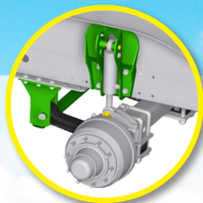
Hydro-Tridem suspension
