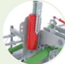
Variflex: continuous modulation of the tine pressure by hydraulic adjustment using multiple compensation cylinders and one or two central cylinders with graduated mark.
