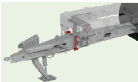
Steel drawbar guide for front suspension , with greasing points and adjustable by 4 pressure screws.
